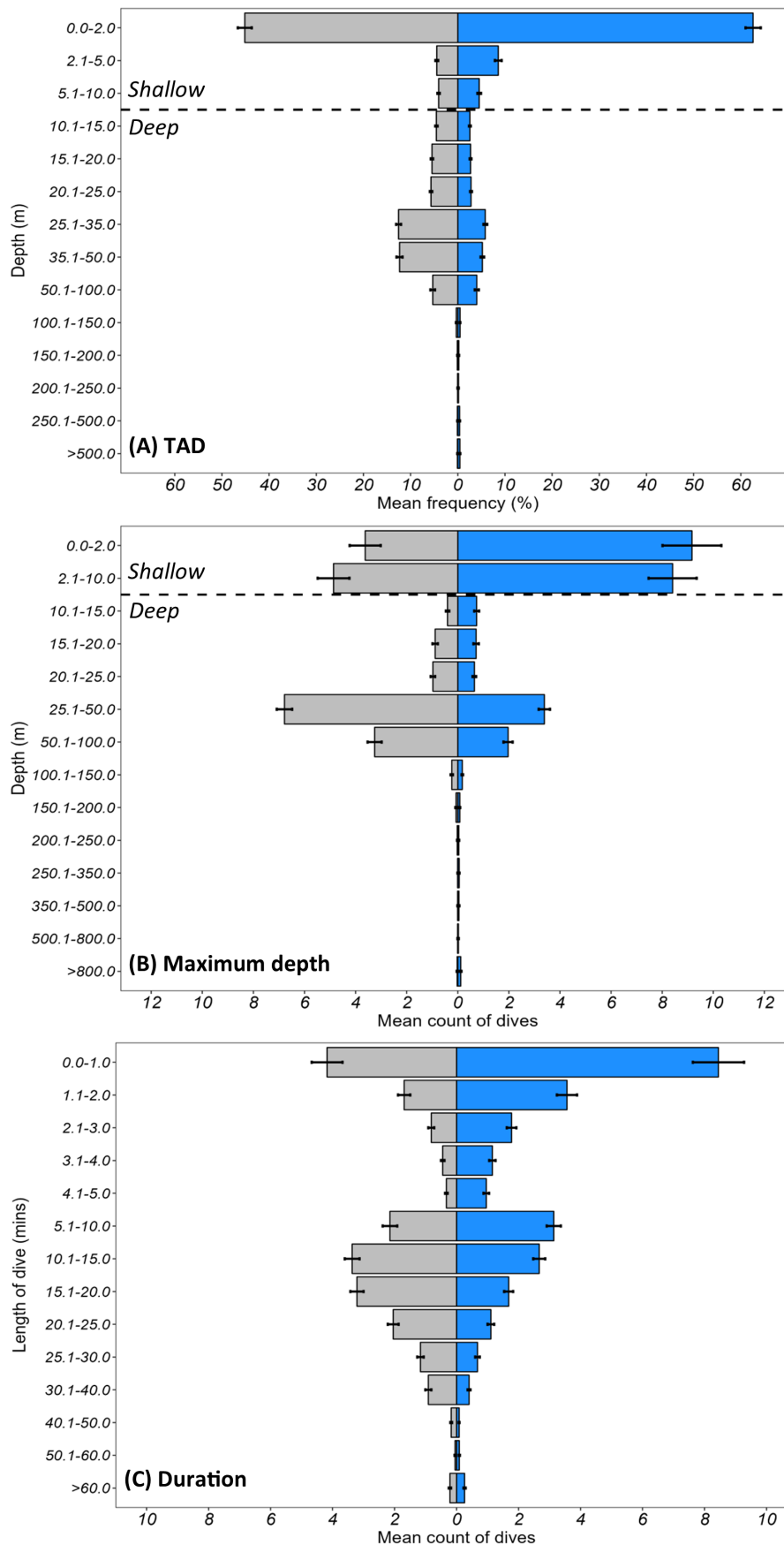
Fig. 3. Dive summary histograms for (A) Time-at-Depth (TAD), (B) maximum dive depth, and (C) dive duration of leatherback turtles ( n = 6 ). Mean \pm standard error split by night (grey bars) and day (blue bars). Horizontal dashed lines: separation between 'shallow' and 'deep' dive categories
